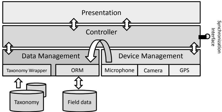
Fig. 1. Four-tier architecture of DiversityMobile
