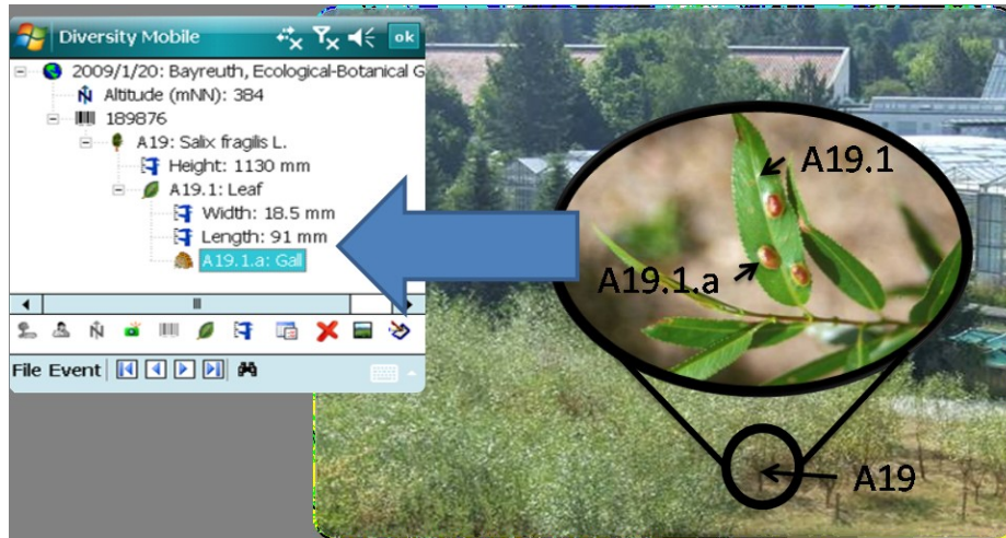
Fig. 3. Exemplary data retrieval of the scenario discussed in Chapter 4
