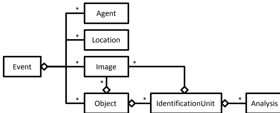
Fig. 2. Simplified version of the DiversityCollection data model as applied in the current DiversityMobile prototype
